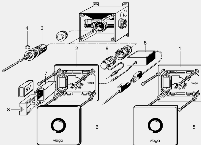
Pokrivna ploča Visign for More 100 - metal, staklo - Sl. 5 Model 8351.8
